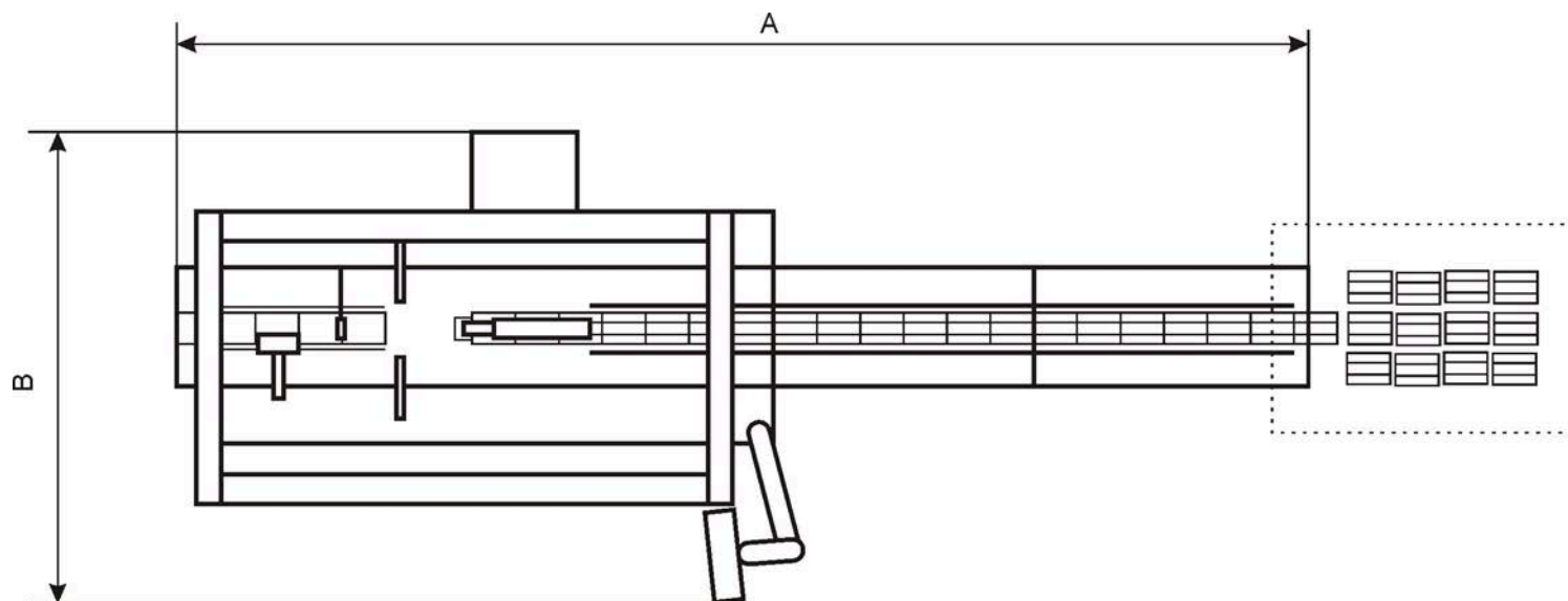
Floor plan for Single-Head Bander BD
